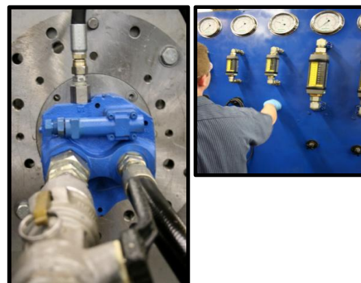
HYDRAULIC LOAD TEST STAND
